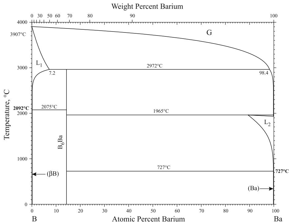
Fig. 1 B-Ba phase diagram
